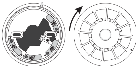
Fig. 4 Fit the detector unit onto the base (as per figure) then twist
